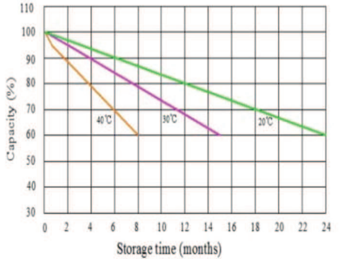
Self-discharge characteristic
