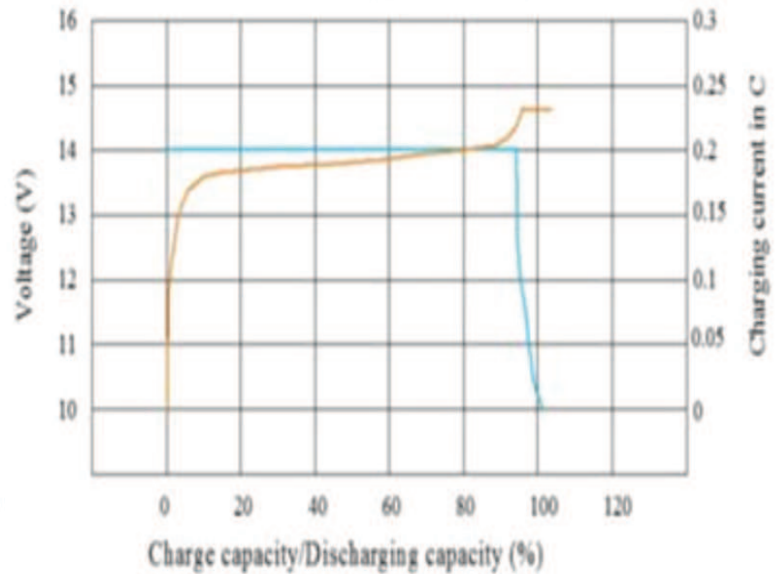
0.2C CC-CV charge characteristic
