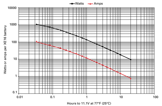
Figure A-8: XE16 discharge data to 11.1V at 77°F (25°C)
