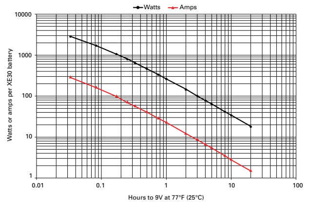
Figure A-9: XE30 discharge data to 9V at 77°F (25°C)
